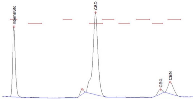
Chromatogram of Cannabinoid Profile
